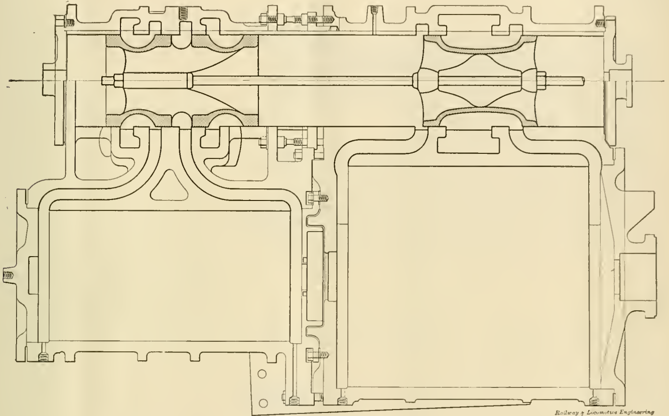
CYLINDERS AND VALVES OF BALDWIN TANDEM—SEE PAGE 274 OF MAY NUMBER.
